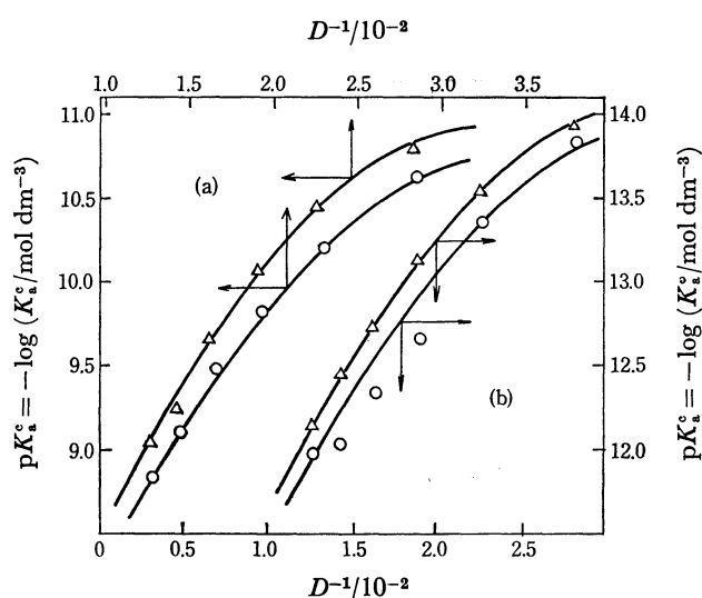
Fig. 4. Dependence of the acid-dissociation constants, K_a^* , of HEB (a) and PAR (b) on the dielectric constant of the medium at 25 °C and I = 0.1 \text{ mol dm}^{-3} ( \text{KNO}_3 ). \circ : The plot of \text{p}K_a^*(k) vs. D^{-1} . \triangle : The plot of \text{p}K_a^*(s) vs. D^{-1} .
