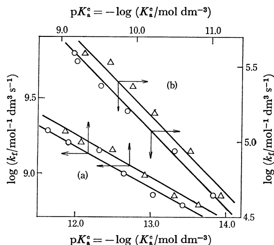
Fig. 6. Dependence of the log k_f on the pK_a^* of HEB (a) and PAR (b) in dioxane-water media at 25 °C and I = 0.1 \text{ mol dm}^{-3} ( \text{KNO}_3 ). ○: The plot of log k_f vs. pK_a^*(k) . △: The plot of log k_f vs. pK_a^*(s) .
